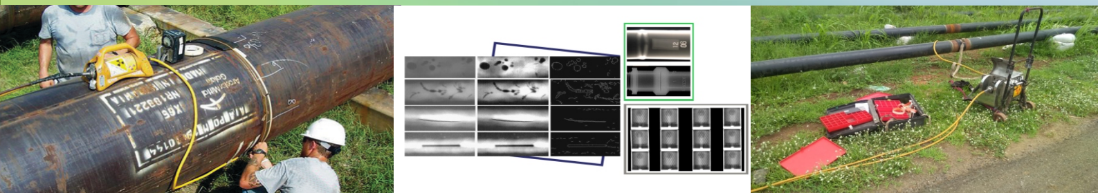
Industrial Radiography Testing (Gamma Ray & X Ray)
